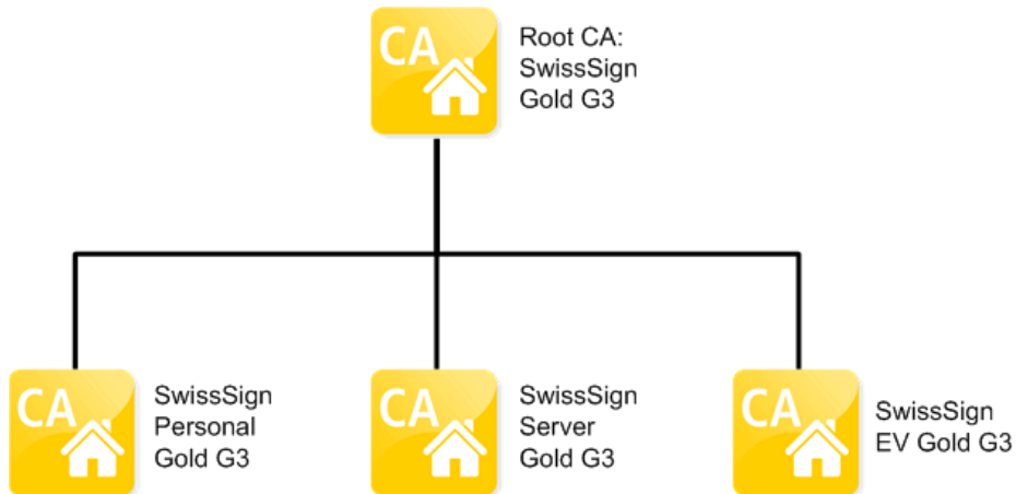
Figure 3: Gold CA Hierarchy G3
