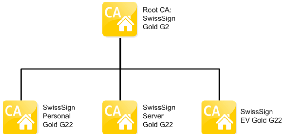
Figure 2: Gold CA Hierarchy G22
