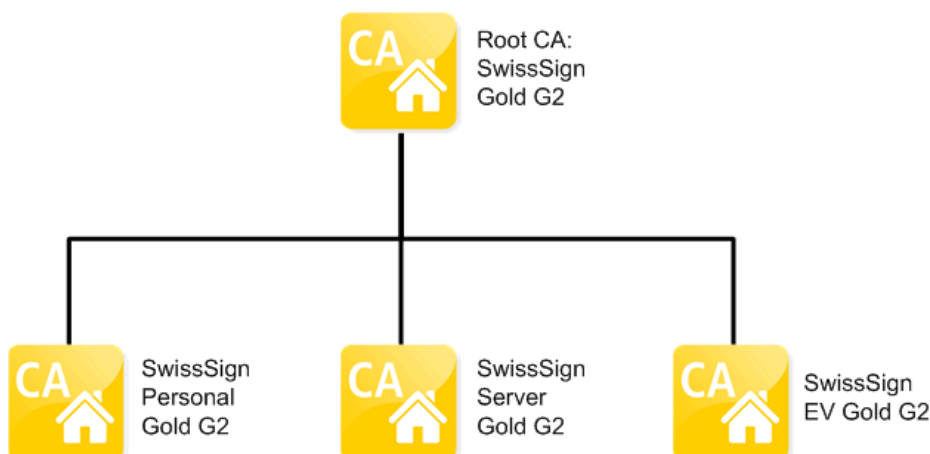
Figure 1: Gold CA Hierarchy G2
